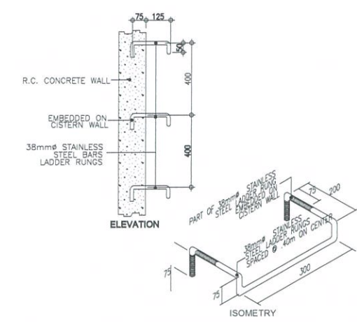
4 TYPICAL LADDER RUNG DETAIL P-18 SCALE: NTS
