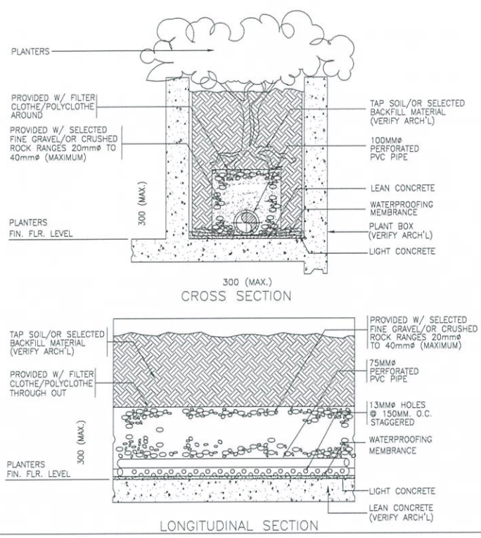
5 PERFORATED PIPE ON PLANTER'S BOX DETAIL P-18 SCALE: NTS
