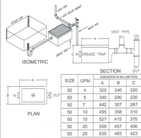
2 GREASE TRAP DETAIL P-18 SCALE: NTS
