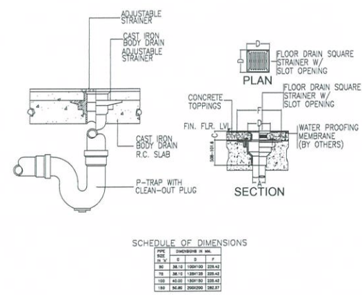
8 FLOOR DRAIN DETAIL P-18 SCALE: NTS
