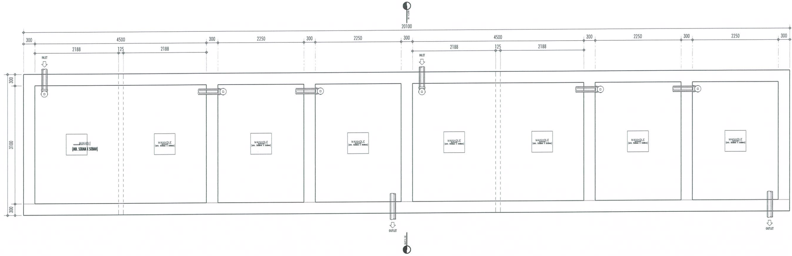
PLAN
