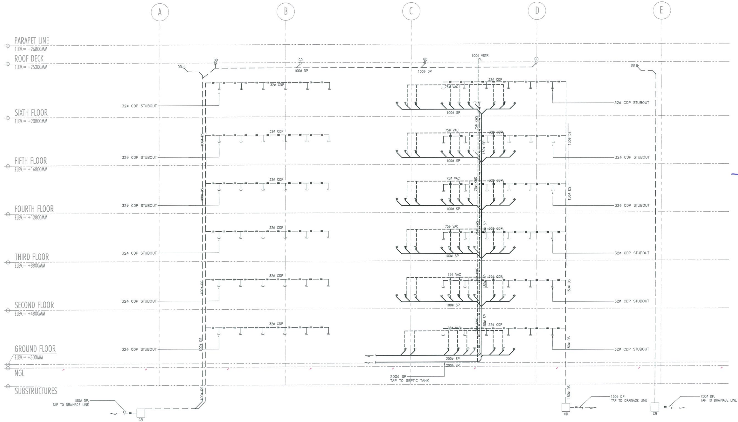
1 P-13 SOIL, WASTE, VENT, STORM AND CONDENSATE DRAIN SCHEMATIC DIAGRAM SCALE: NTS
