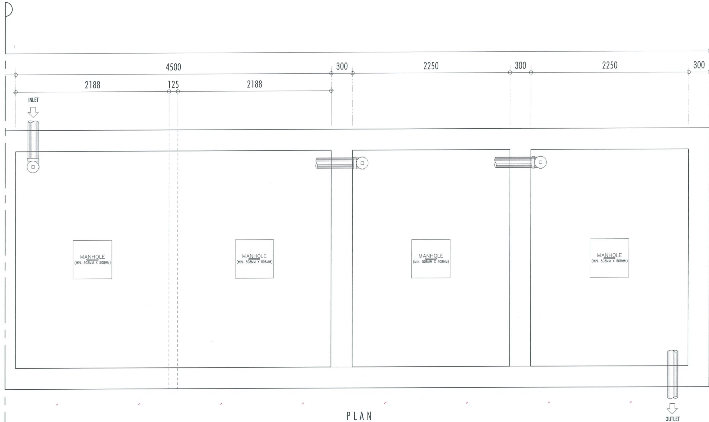
1 P-19 SCALE: NTS SEPTIC TANK DETAILS (PLAN) - II
