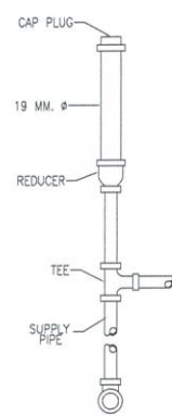
1 AIR CHAMBER DETAIL P-18 SCALE: NTS
