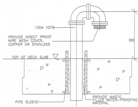
6 VENT STACK THRU ROOF DETAIL P-18 SCALE: NTS
