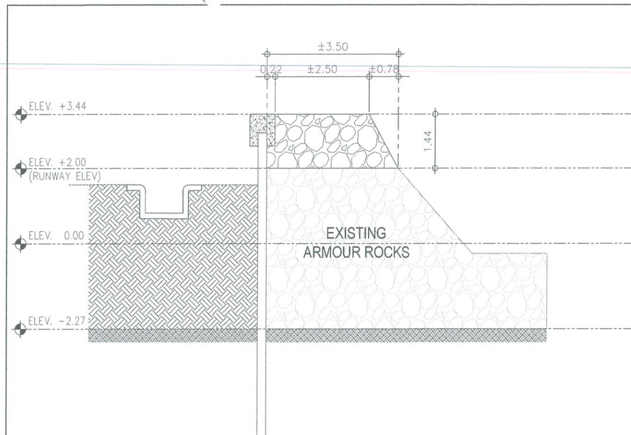
1 C-8/C-8 ARMOUR ROCKS @ STA. 0+220 DETAILED SECTION SCALE: 1:100 M
