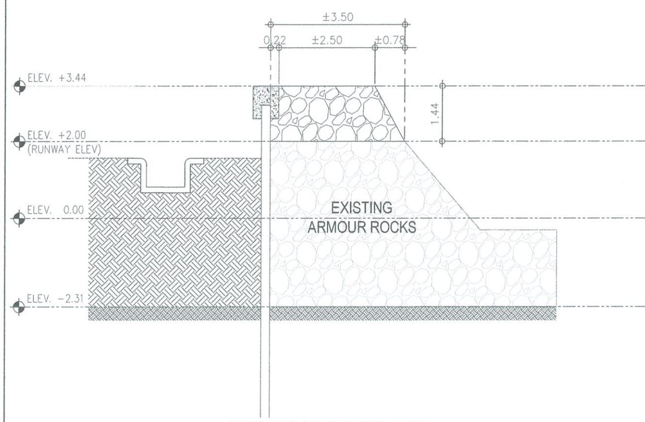
3 C-8/C-8 ARMOUR ROCKS @ STA. 0+260 DETAILED SECTION SCALE: 1:100 M
