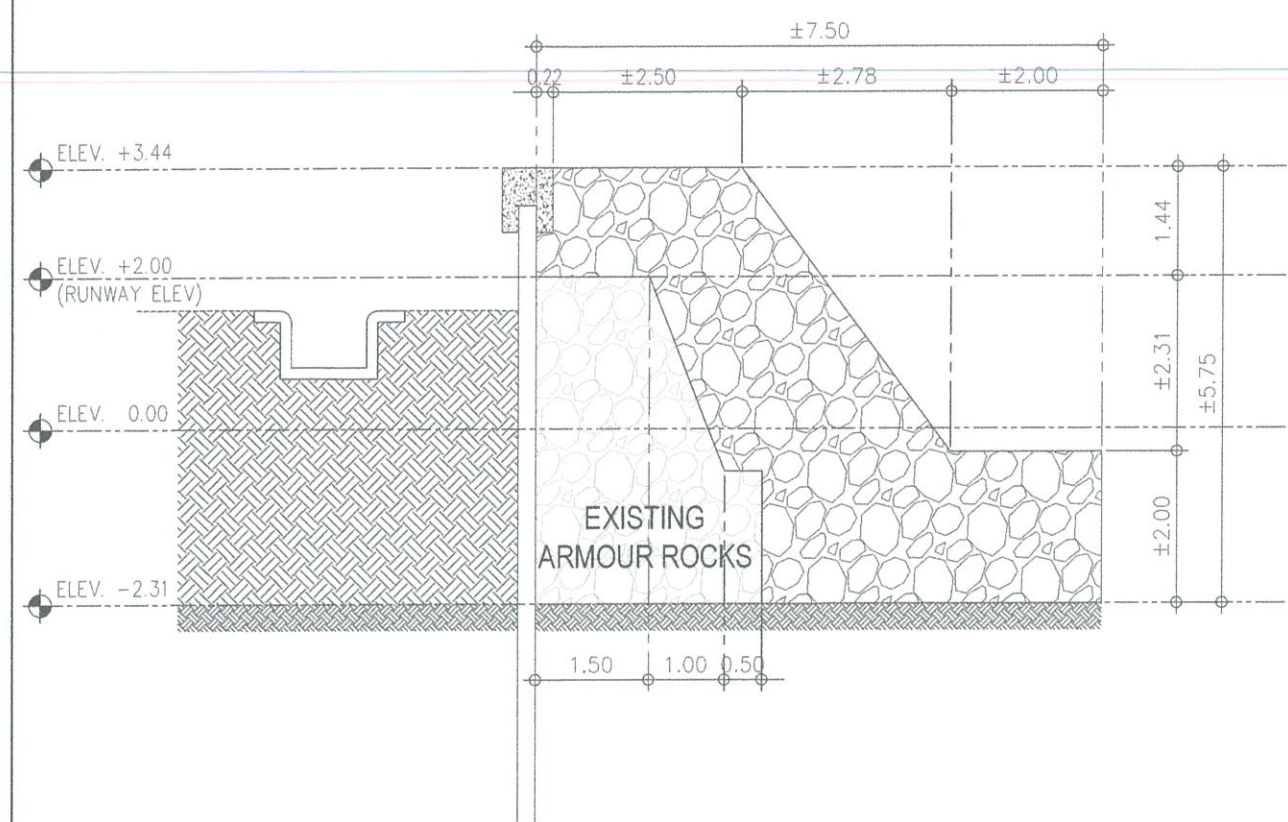
1 C-3 C-3 ARMOUR ROCKS @ STA. 0-160a DETAILED SECTION SCALE: 1:100 M
