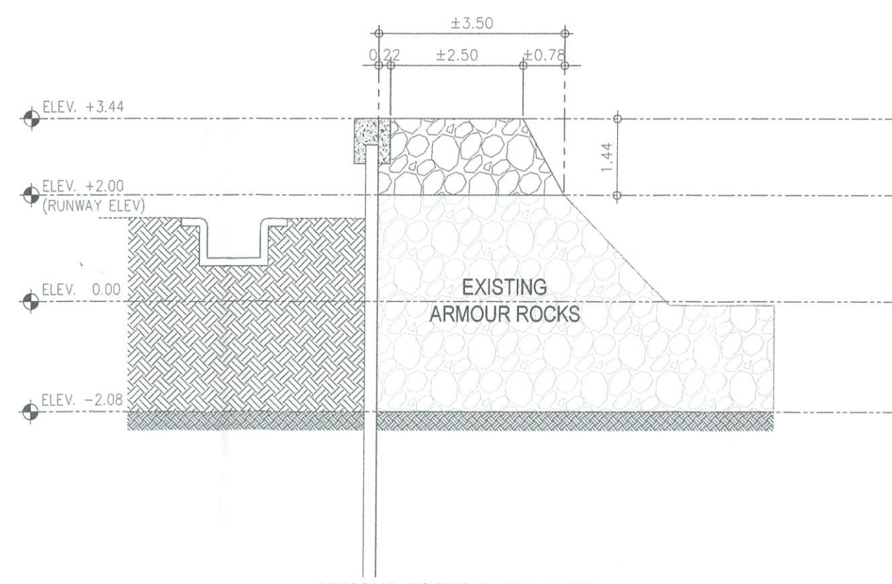
4 C-8/C-8 ARMOUR ROCKS @ STA. 0+280 DETAILED SECTION SCALE: 1:100 M
