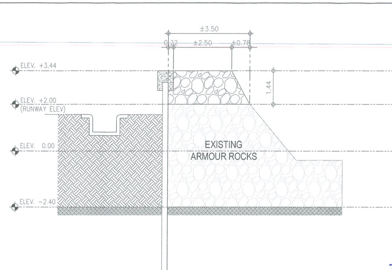
2 C-8/C-8 ARMOUR ROCKS @ STA. 0+240 DETAILED SECTION SCALE: 1:100 M
