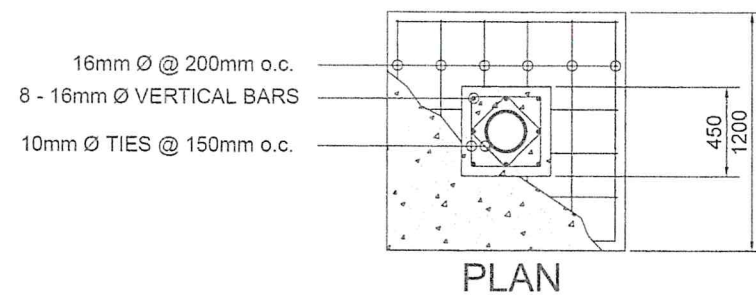
SOLAR STREET LIGHT POST PEDESTAL DETAILS SCALE: 1:20 MTS.
