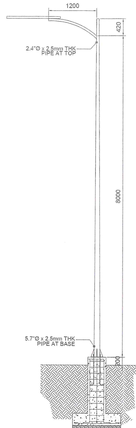
SOLAR STREET LIGHT POST DETAILS SCALE: 1:50 MTS.
