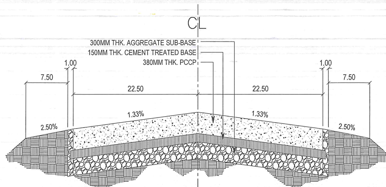
SECTION VIEW W/OUT EXISTING TURNAROUND PAD
