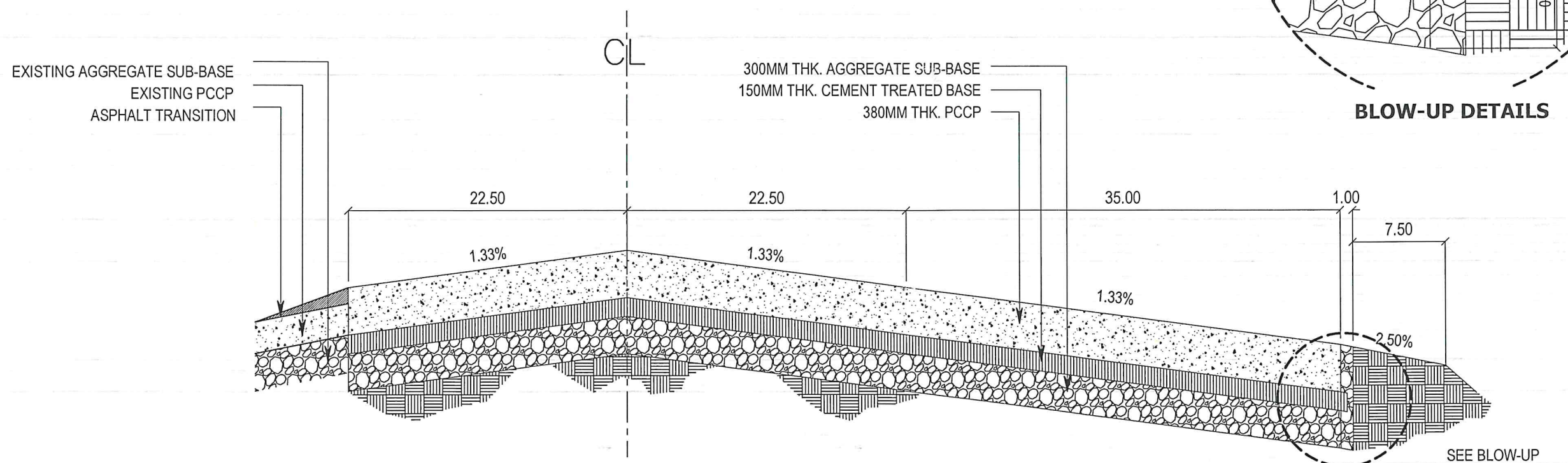
SECTION VIEW ON EXISTING TURNAROUND PAD
