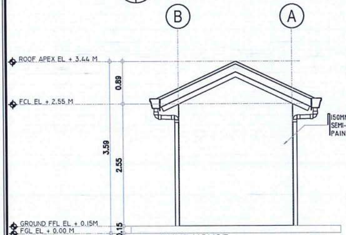
7 PUMP HOUSE REAR ELEVATION SCALE: 1 : 75 M
