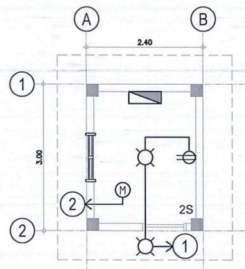
1 PUMP HOUSE LIGHTING AND POWER PLAN SCALE: 1 : 75 M
