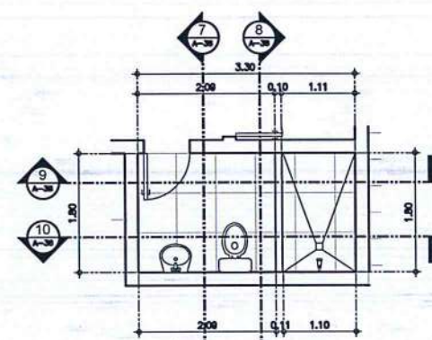
TOILET @ CATC CHIEF OFFICE 6 A-B SCALE: 1 : 50 M
