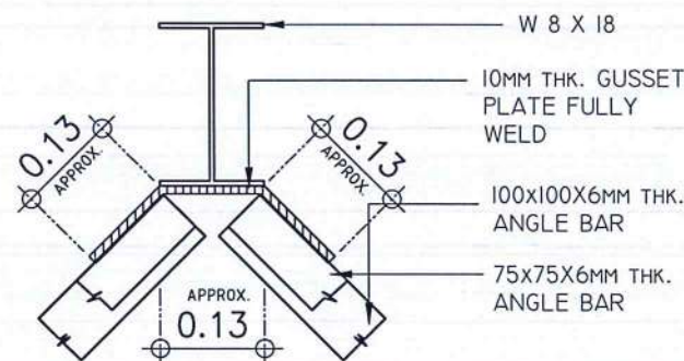
12 S-2 S-2 BRACING BLOW-UP DETAIL SCALE: NTS
