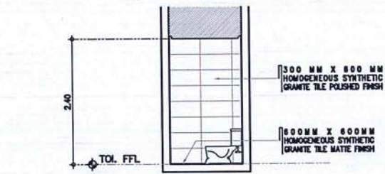
TOILET @ CLINIC DETAILED SECTION A SCALE: 1 : 50 M
