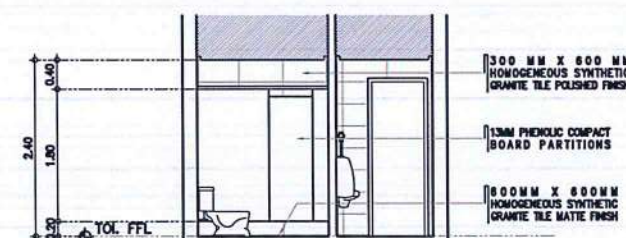
TOILET @ ADMIN OFFICE 4 A-B SCALE: 1 : 50 M
