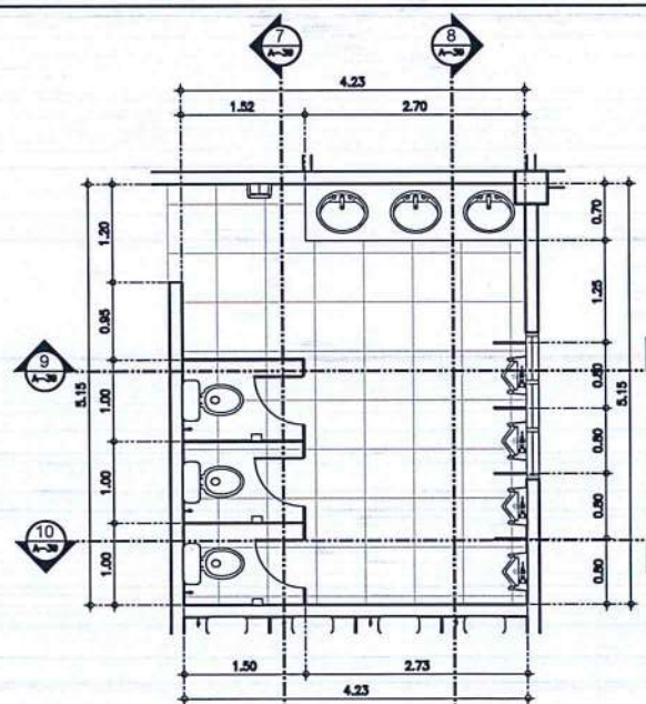
6 MALE TOI. @ GROUND FLR LOBBY A-9 SCALE: 1 : 50 M
