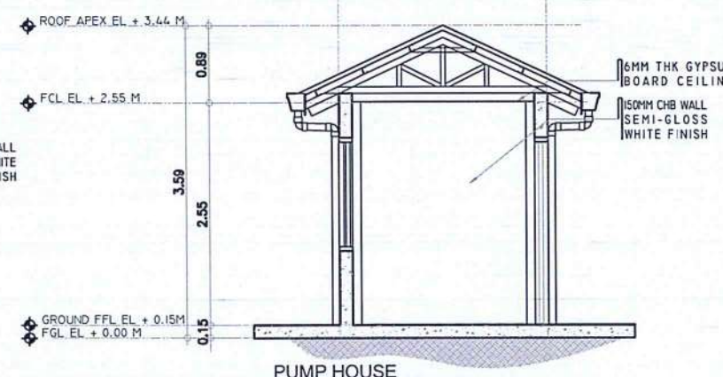
10 PUMP HOUSE SECTION THRU 'A' SCALE: 1 : 75 M
