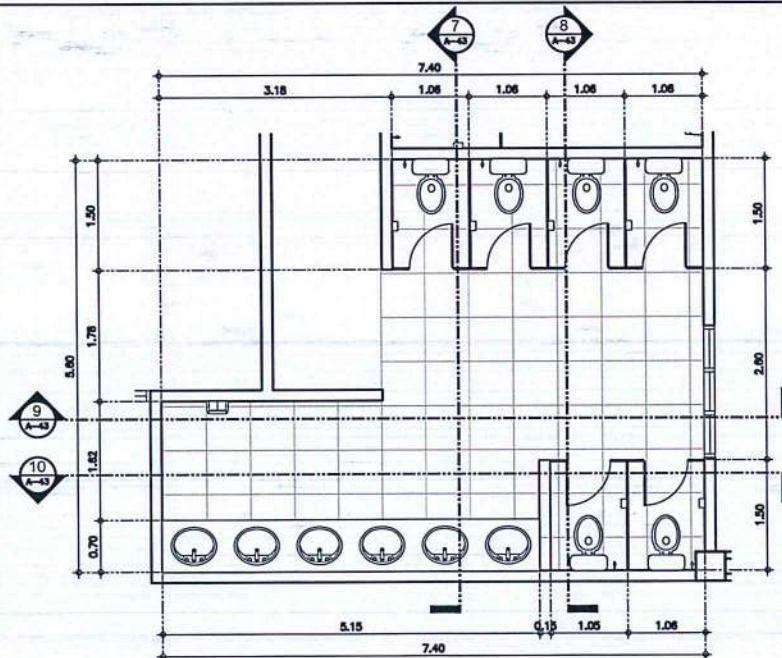
6 FEMALE TOILET @ 2ND FLR LOBBY A-13 DETAILED PLAN SCALE: 1 : 50 M
