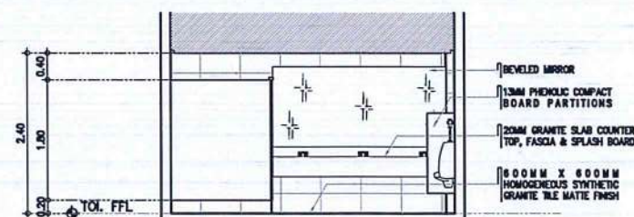
9 MALE TOI. @ GROUND FLR LOBBY A-9 SCALE: 1 : 50 M
