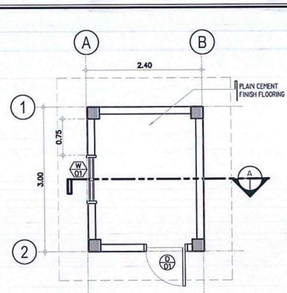
1 PUMP HOUSE PROPOSED FLOOR PLAN SCALE: 1 : 75 M
