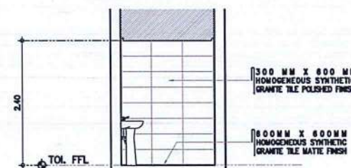
TOILET @ CATC CHIEF OFFICE 7 A-B SCALE: 1 : 50 M
