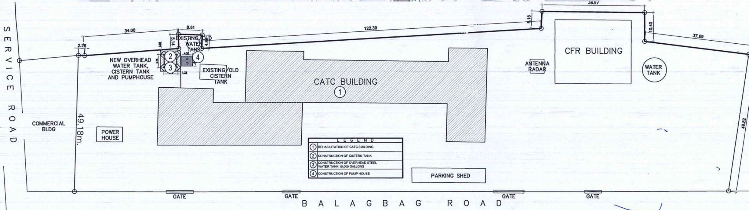
1 SITE DEVELOPMENT & LOCATION PLAN SCALE: NTS
