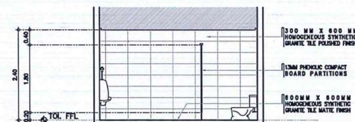
10 MALE TOI. @ GROUND FLR LOBBY A-9 SCALE: 1 : 50 M
