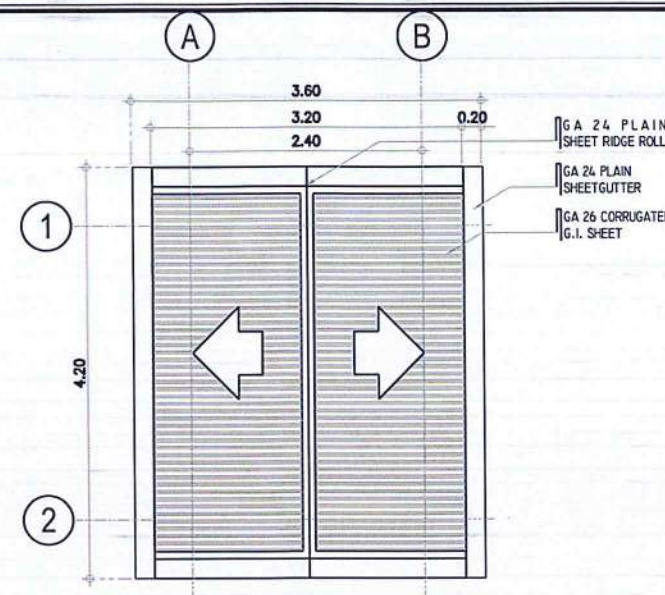
3 PUMP HOUSE ROOF PLAN SCALE: 1 : 75 M
