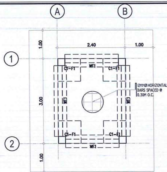
2 PUMP HOUSE FOUNDATION PLAN SCALE: 1 : 75 M
