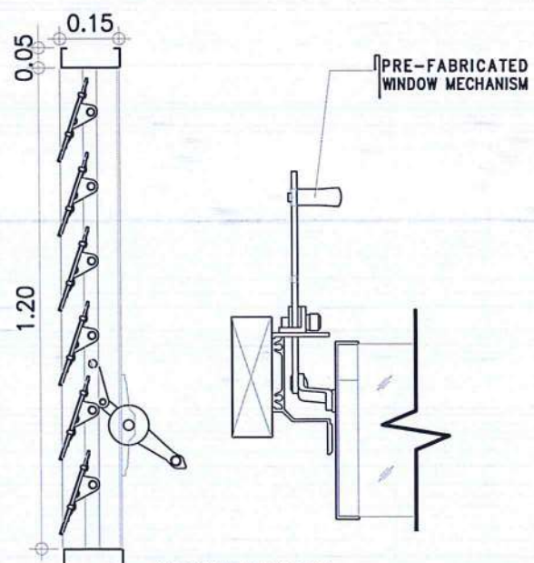
14 JALOUSIE WINDOW BLOW-UP DETAILS SCALE: NTS
