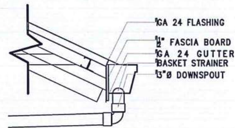
13 PUMP HOUSE GUTTER DETAILS SCALE: NTS
