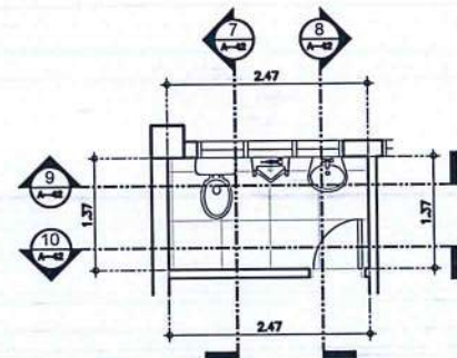
TOILET @ CLINIC DETAILED PLAN SCALE: 1 : 50 M
