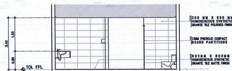
7 FEMALE TOILET @ 2ND FLR LOBBY A-13 DETAILED SECTION A SCALE: 1 : 50 M
