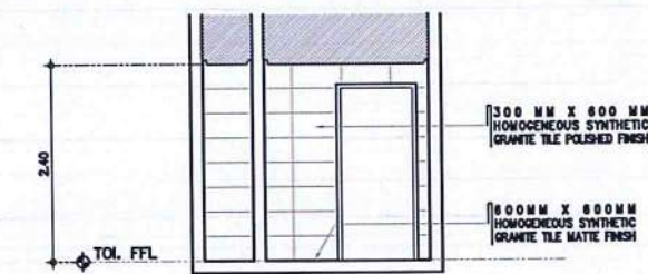
PWD TOILET @ CAFETERIA DETAILED SECTION C SCALE: 1 : 50 M
