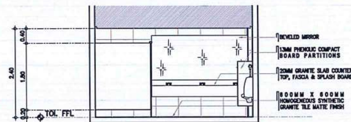
4 MALE TOILET @ 2ND FLR LOBBY A-13 DETAILED SECTION C SCALE: 1 : 50 M
