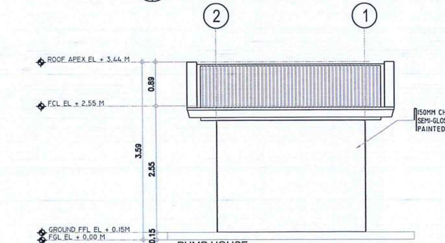
8 PUMP HOUSE RIGHT SIDE ELEVATION SCALE: 1 : 75 M
