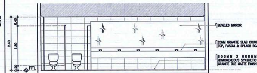
10 FEMALE TOILET @ 2ND FLR LOBBY A-13 DETAILED SECTION D SCALE: 1 : 50 M
