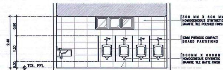
8 MALE TOI. @ GROUND FLR LOBBY A-9 SCALE: 1 : 50 M
