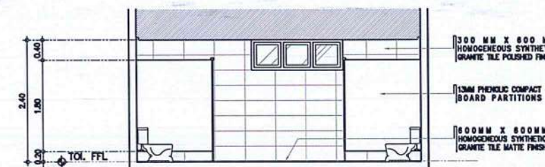
8 FEMALE TOILET @ 2ND FLR LOBBY A-13 DETAILED SECTION B SCALE: 1 : 50 M
