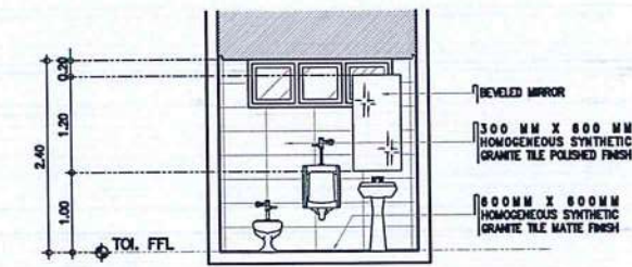
TOILET @ CLINIC DETAILED SECTION C SCALE: 1 : 50 M
