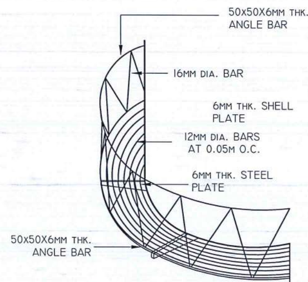
13 S-2 S-2 CATWALK BLOW-UP DETAIL SCALE: NTS
