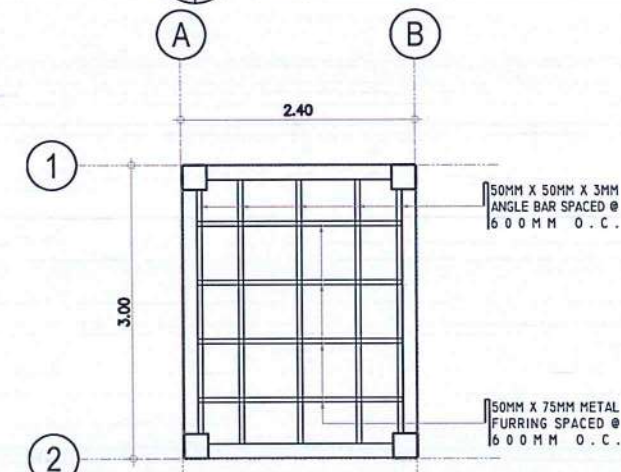
9 PUMP HOUSE CEILING FRAMING PLAN SCALE: 1 : 75 M
