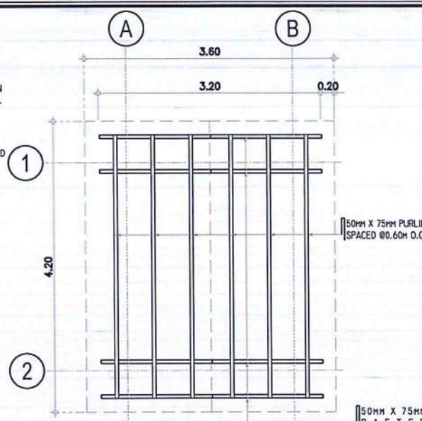
4 PUMP HOUSE ROOF FRAMING PLAN SCALE: 1 : 75 M
