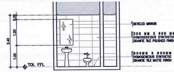
PWD TOILET @ CAFETERIA DETAILED SECTION D SCALE: 1 : 50 M
