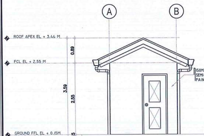
5 PUMP HOUSE FRONT ELEVATION SCALE: 1 : 75 M
