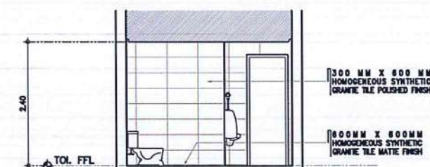
TOILET @ ADMIN OFFICE 5 A-B SCALE: 1 : 50 M
