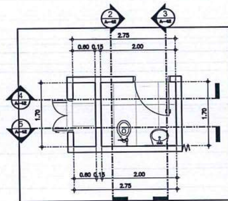
PWD TOILET @ CAFETERIA DETAILED PLAN SCALE: 1 : 50 M
