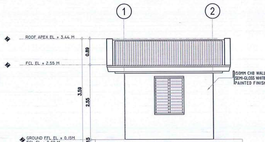
6 PUMP HOUSE LEFT SIDE ELEVATION SCALE: 1 : 75 M
