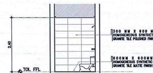
TOILET @ CATC CHIEF OFFICE 8 A-B SCALE: 1 : 50 M
