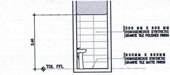
TOILET @ CLINIC DETAILED SECTION B SCALE: 1 : 50 M
