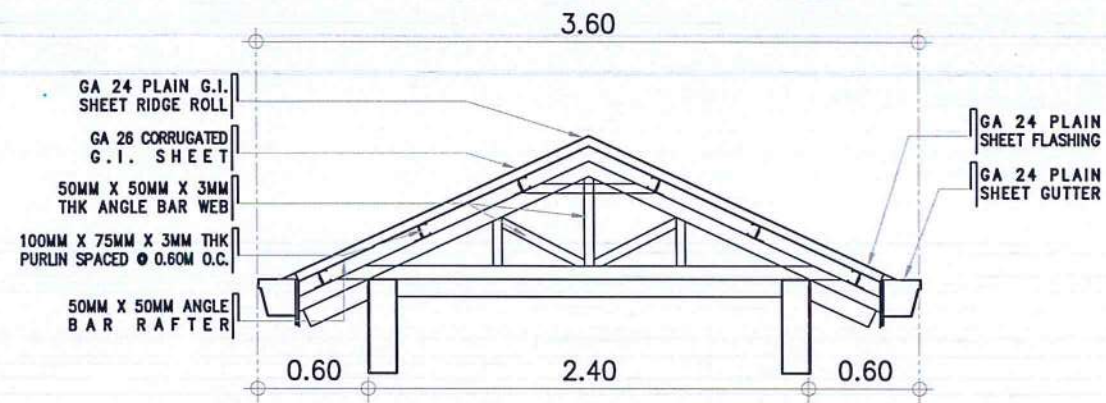
12 PUMP HOUSE TRUSS DETAILS SCALE: 1 : 40 M
