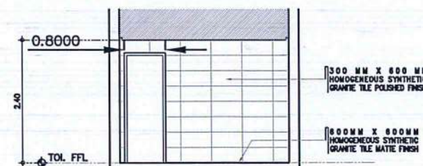
TOILET @ CATC CHIEF OFFICE 9 A-B SCALE: 1 : 50 M
