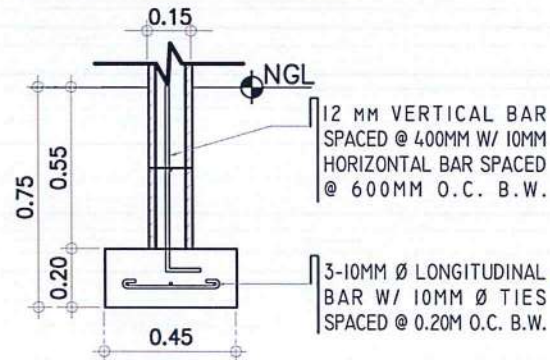
16 PUMP HOUSE WALL FOOTING DETAILS SCALE: 1 : 25 M
