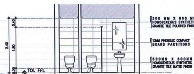
TOILET @ ADMIN OFFICE 2 A-B SCALE: 1 : 50 M
