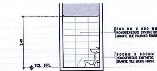
PWD TOILET @ CAFETERIA DETAILED SECTION A SCALE: 1 : 50 M
