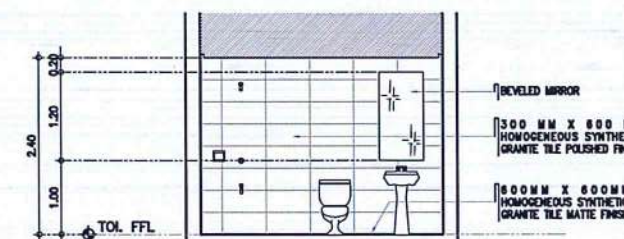
TOILET @ CATC CHIEF OFFICE 10 A-B SCALE: 1 : 50 M
