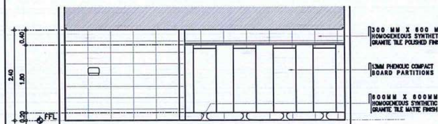
9 FEMALE TOILET @ 2ND FLR LOBBY A-13 DETAILED SECTION C SCALE: 1 : 50 M
