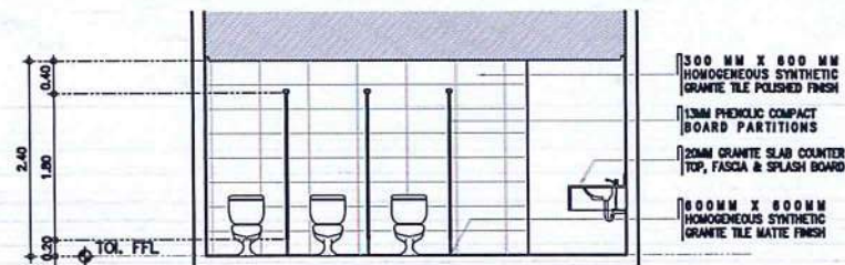
2 MALE TOILET @ 2ND FLR LOBBY A-13 DETAILED SECTION A SCALE: 1 : 50 M
