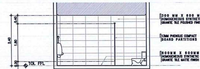
5 MALE TOILET @ 2ND FLR LOBBY A-13 DETAILED SECTION D SCALE: 1 : 50 M
