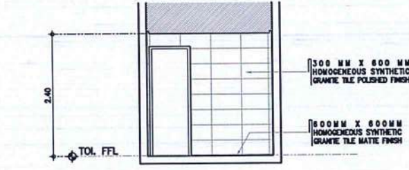
TOILET @ CLINIC DETAILED SECTION D SCALE: 1 : 50 M
