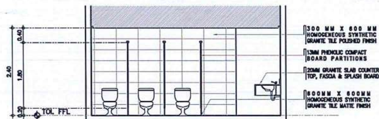
7 MALE TOI. @ GROUND FLR LOBBY A-9 SCALE: 1 : 50 M
