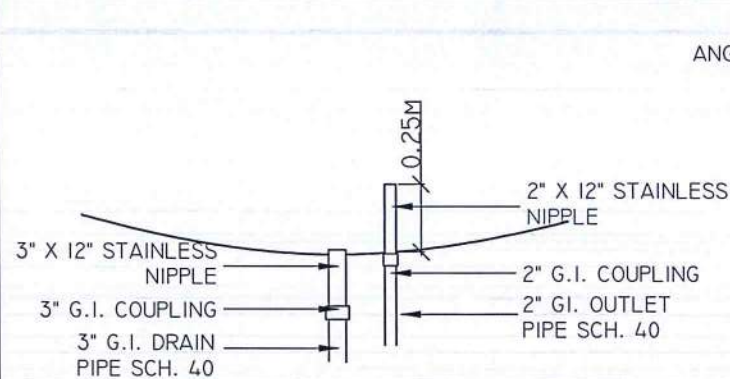
10 S-2 S-2 PIPE BLOW-UP DETAIL SCALE: NTS
