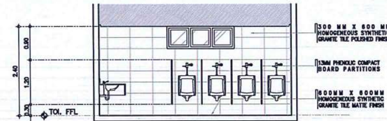
3 MALE TOILET @ 2ND FLR LOBBY A-13 DETAILED SECTION B SCALE: 1 : 50 M
