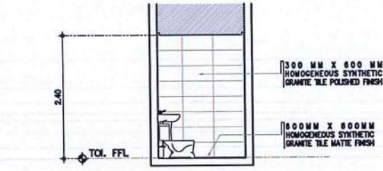
PWD TOILET @ CAFETERIA DETAILED SECTION B SCALE: 1 : 50 M
