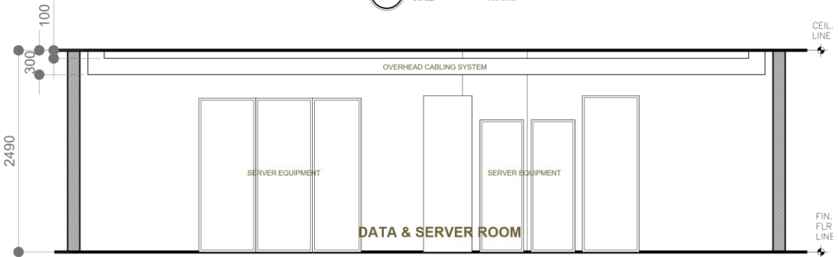
MISD OFFICE INTERIOR ELEVATION "A" SCALE: 1:50 MTS.
