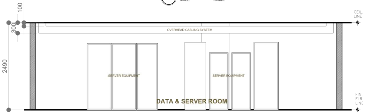
MISD OFFICE INTERIOR ELEVATION "A" SCALE: 1:50 MTS.
