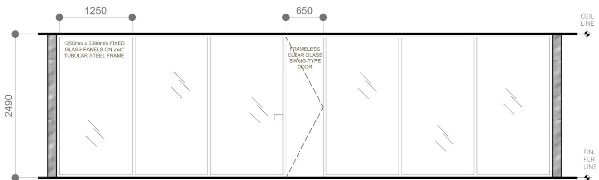
MISD OFFICE INTERIOR ELEVATION "B" SCALE: 1:50 MTS.
