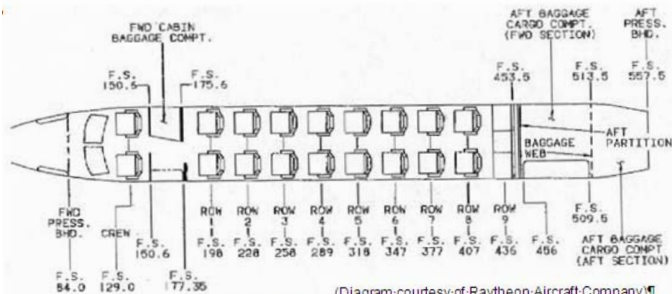
FIGURE 3-1. SAMPLE AIRCRAFT INTERIOR SEATING DIAGRAM
