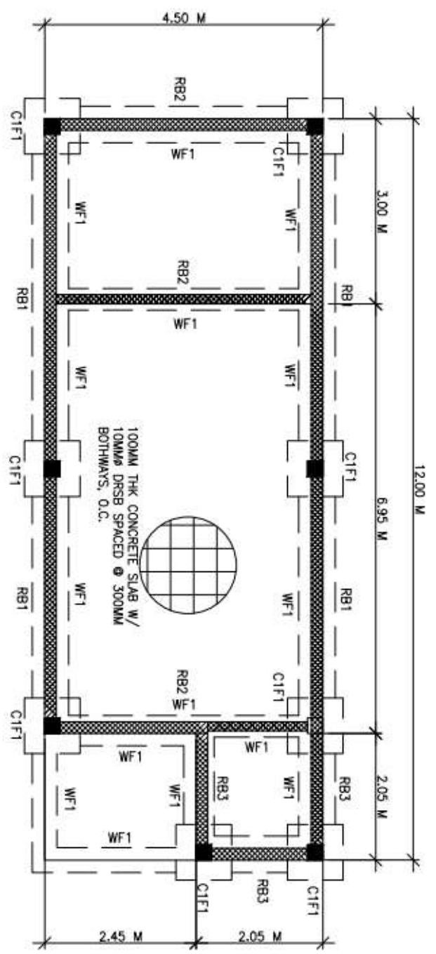
FOUNDATION PLAN
