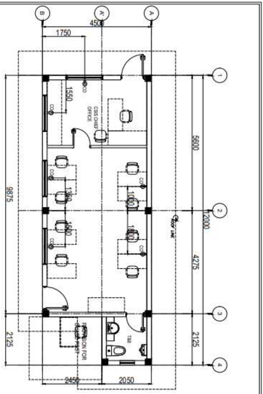
1 CSIS OFFICE POWER LAYOUT SCALE: 1/32" = 1'-0"
