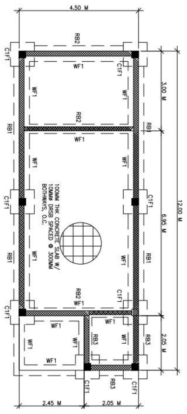
FOUNDATION PLAN
