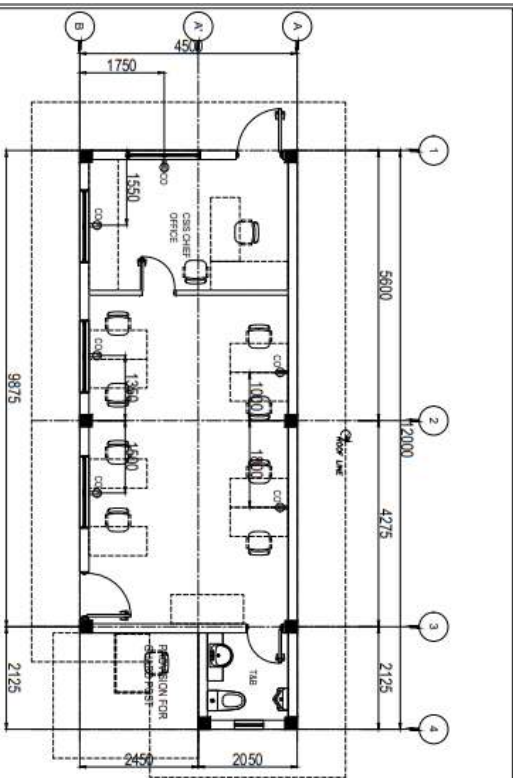
1 CSIS OFFICE POWER LAYOUT SCALE: 1/32" AS2
