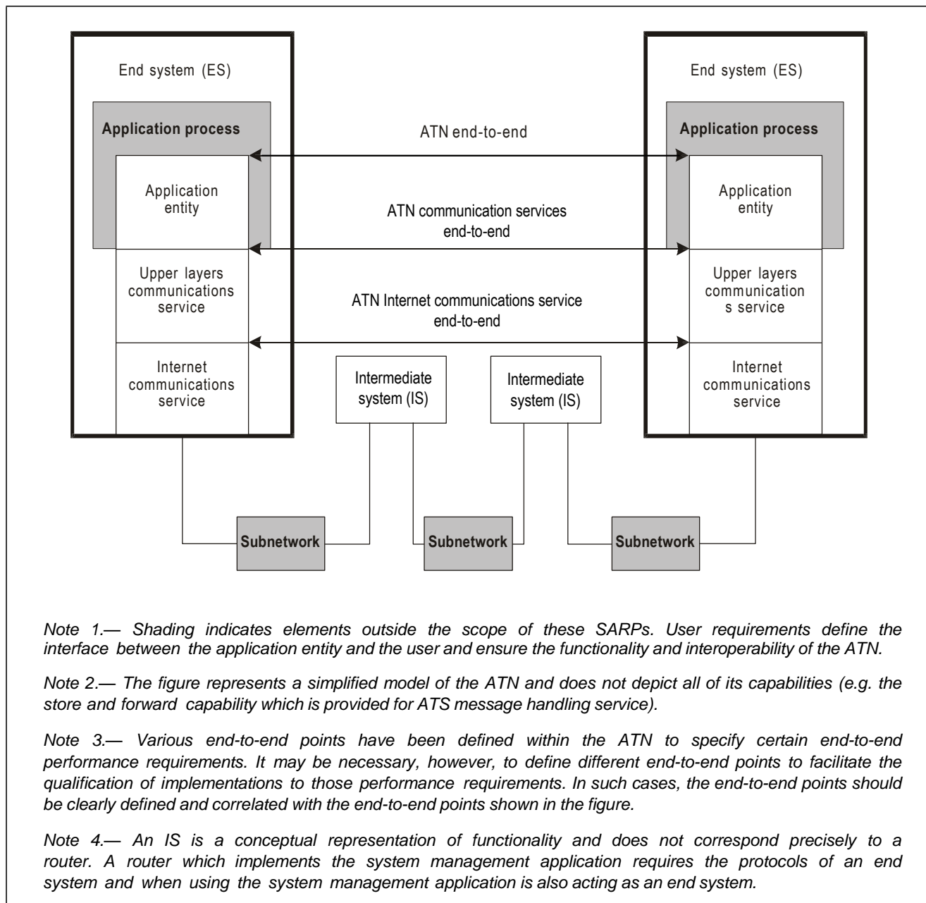
Figure 7.3-3 Conceptual model of the ATN
