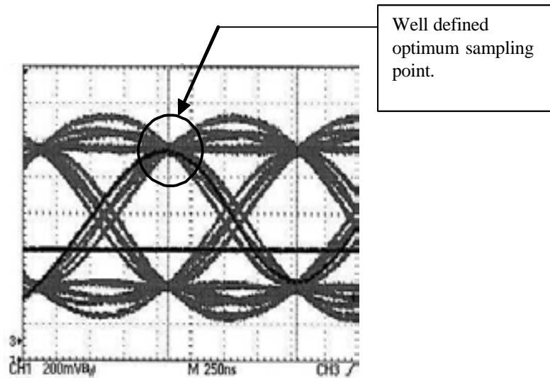
Figure 7.12-3. Ideal eye diagram
