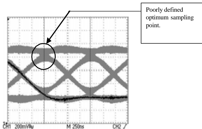
Figure 7.12-4. Distorted eye diagram
