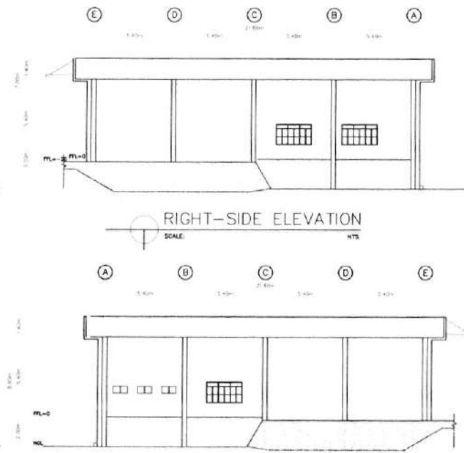
LEFT-SIDE ELEVATION SCALE: NTS.
