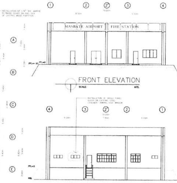
FRONT ELEVATION SCALE: NTS.
