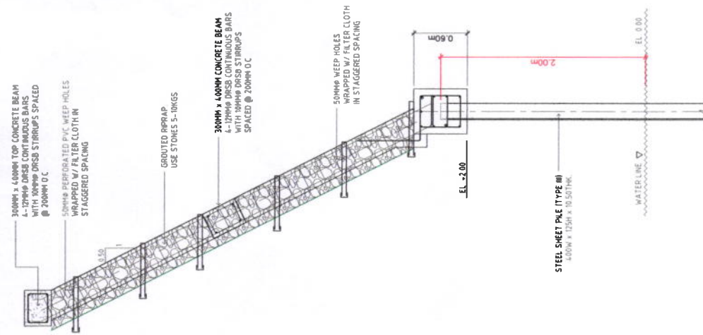
DETAIL OF WEEP HOLES
