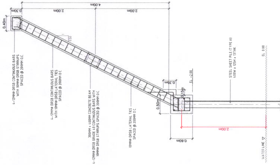
REBAR DETAIL OF PILE COPING & GROUDED RIPRAP WALL
